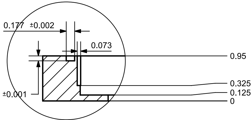
DETAIL B SCALE 1:1
